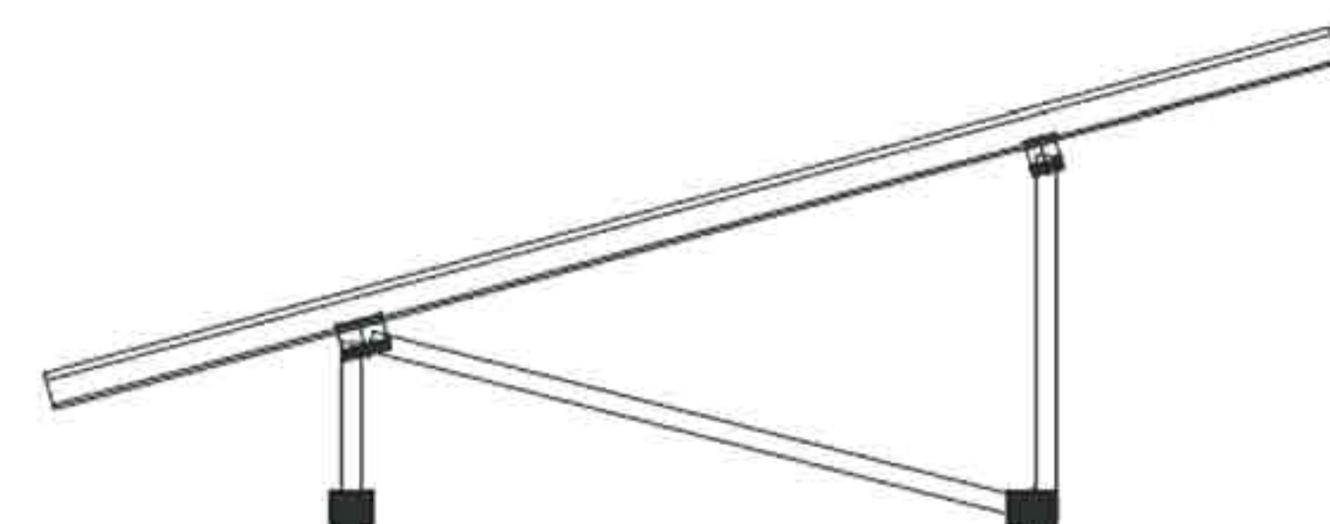
Pre-assembled N Support
