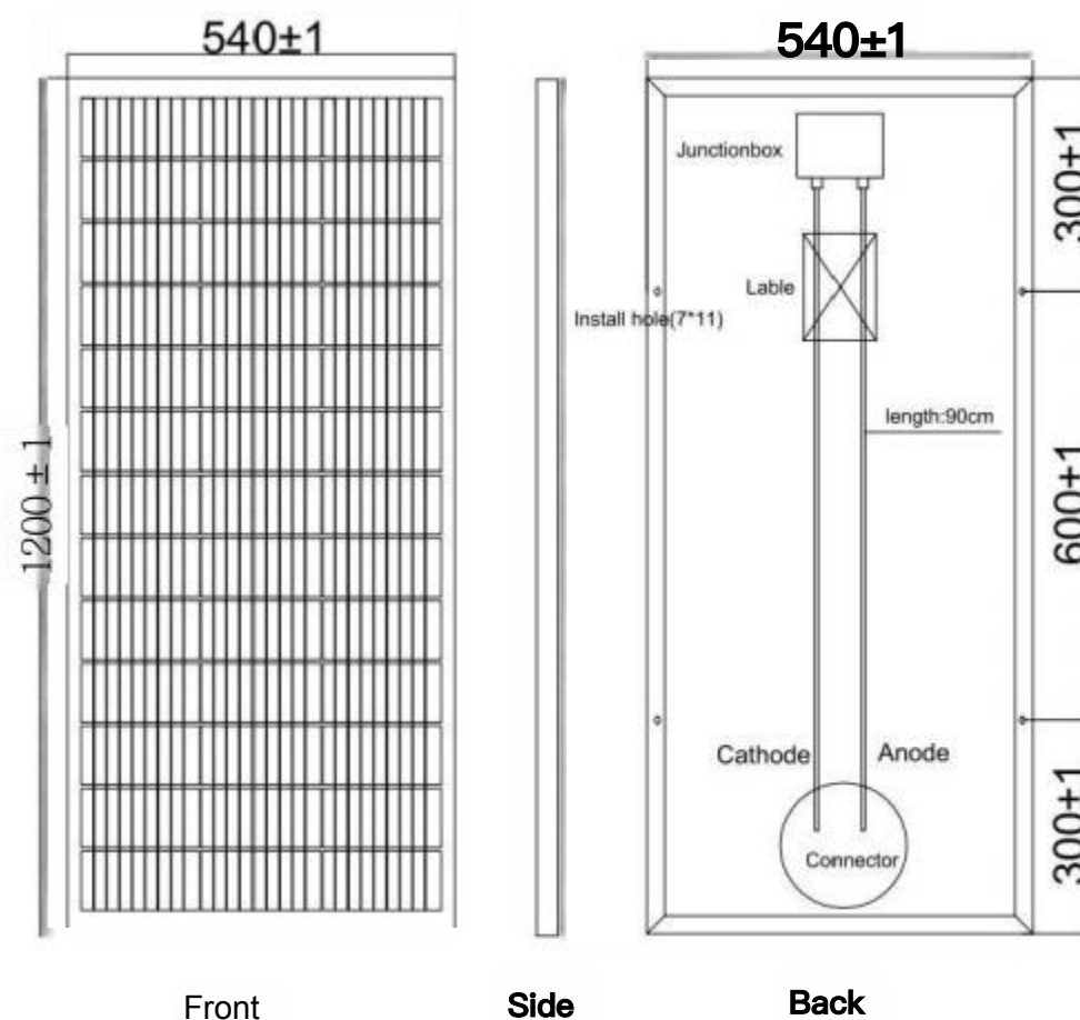
120W Mono solar Panel (540*1200*30*25mm)
