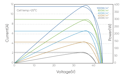
I-V/P-V Curve at Different Temperature (390W)
