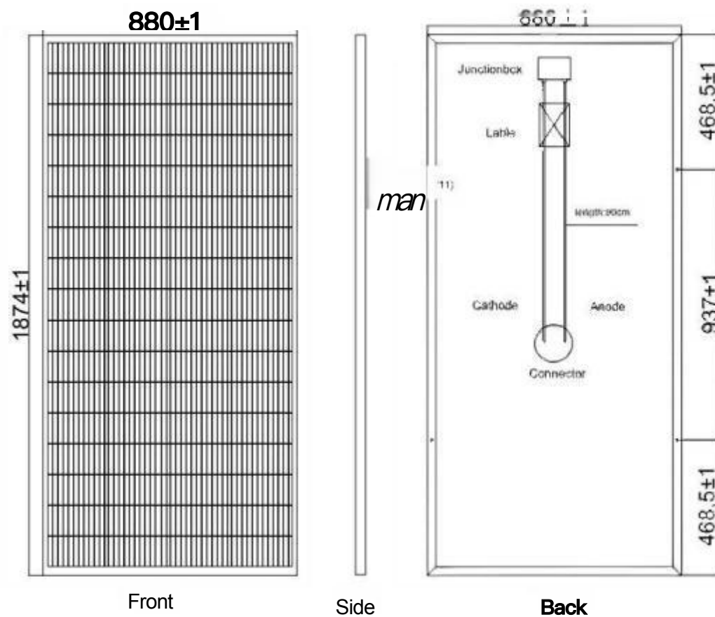
360W Mono solar Panel (880*1874*35*30mm)
