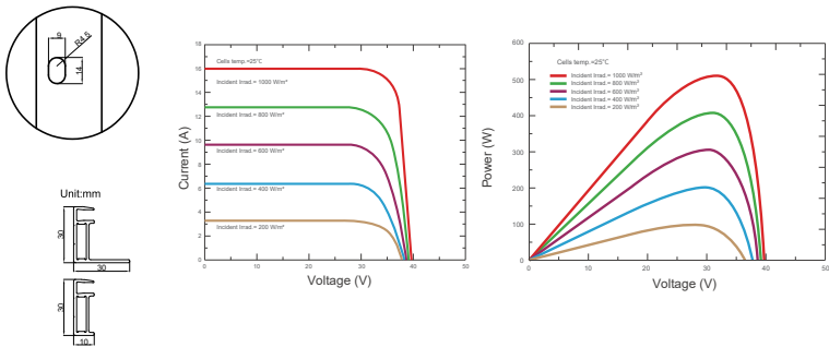
Current-Voltage & Power-Voltage Curves (SKT510M12-108D4)
