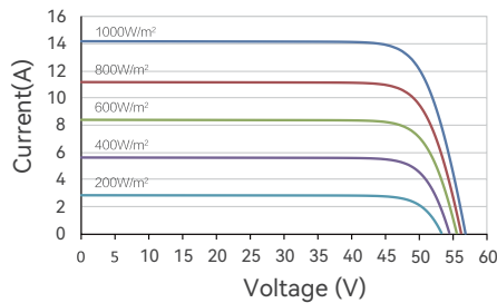
Current-Voltage(635W)
