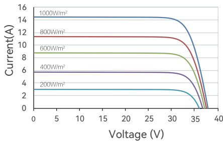
Current-Voltage(450W)
